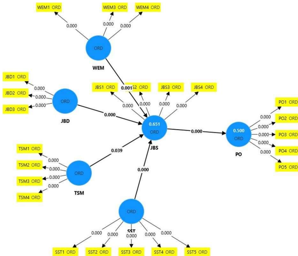
Figure 2: Structural Equation Model (SEM)
